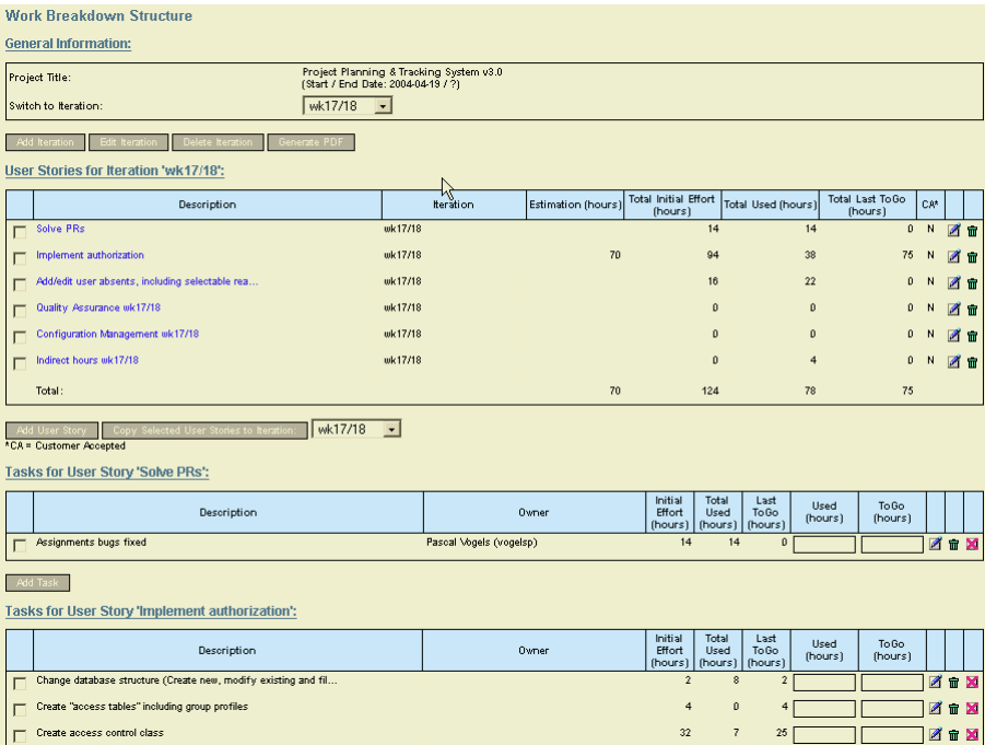
Fig. 1. Part of Web page showing the user stories and tasks for a particular iteration together with their initial and current estimations and currently spent effort
